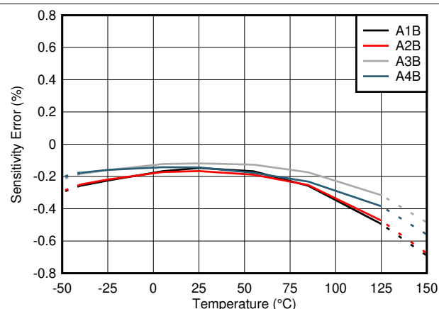
Figure 44. Sensitivity Drift Across Temperature (B Variants)
