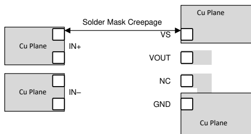
Figure 59. Layout for System Creepage Requirements
