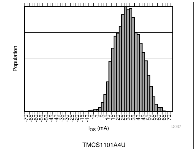
Figure 16. Input Offset Current Production Distribution
