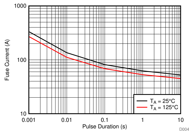
Figure 40. Single-Pulse Leadframe Capability
