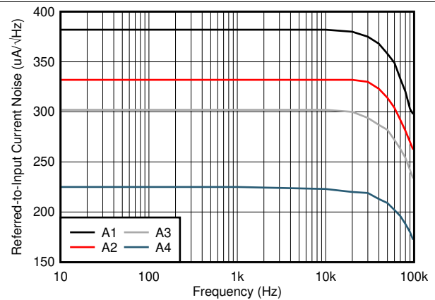
Figure 22. Input-Referred Noise vs Frequency
