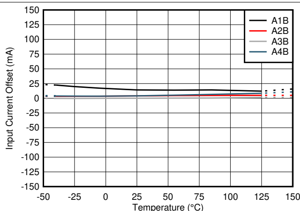
Figure 42. Offset Error Drift Across Temperature (B Variants)
