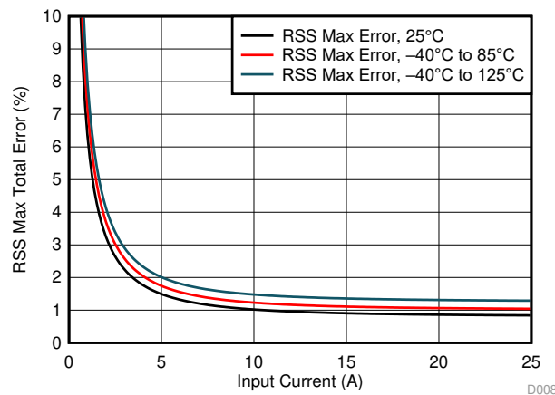
Figure 55. RSS Error vs Input Current
