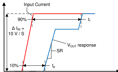
Figure 34. Current Overload Transient Response
