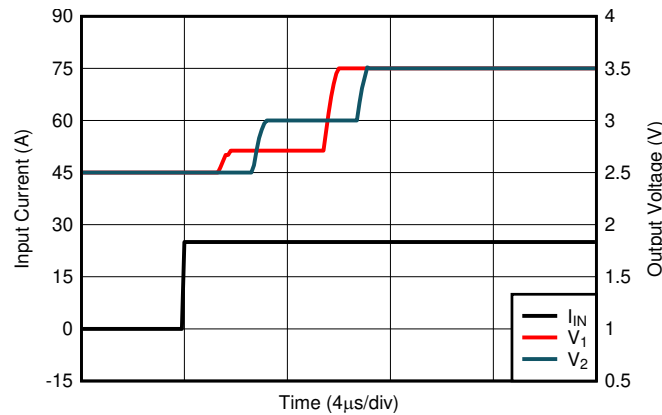
Figure 52. Transient Response to Input-Current Step Sufficient for 1-V Output Swing
