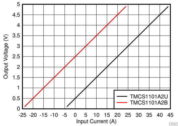
Figure 54. Output Voltage Relationship to Input Current for TMCS1101A2B and TMCS1101A2U
