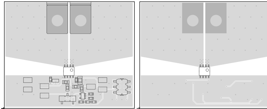
Figure 60. Recommended Board Top (Left) and Bottom (Right) Plane Layout
