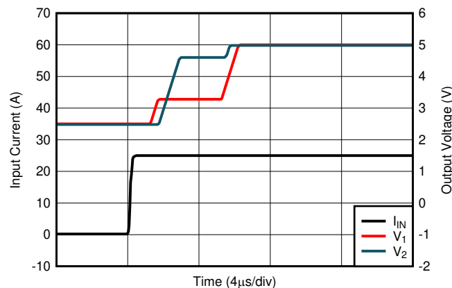
Figure 53. Transient Response to a Large Input Current Step
