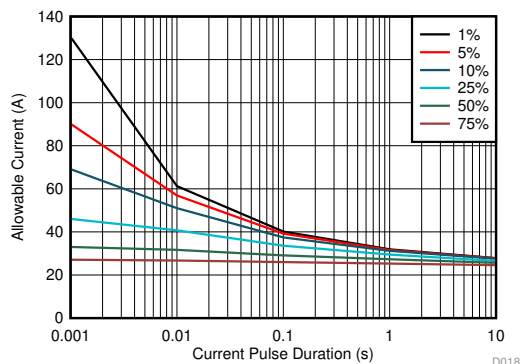
Figure 36. Maximum Repetitive Pulsed Current vs Pulse Duration
