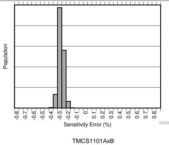
Figure 7. Sensitivity Error Production Distribution
