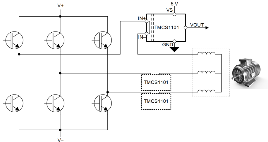
Figure 56. Inline Motor Phase Current Sensing
