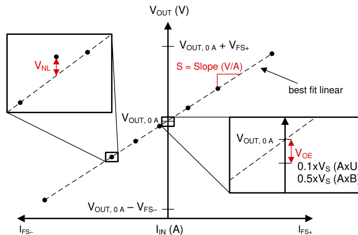
Figure 31. Sensitivity, Offset, and Nonlinearity Error
