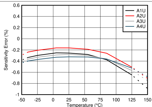
Figure 45. Sensitivity Drift Across Temperature (U Variants)
