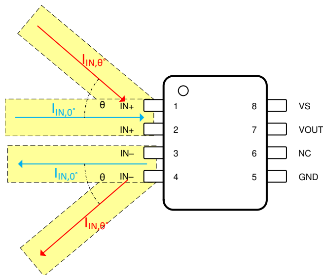
Figure 58. Magnetic Field Generated by Input Current Trace
