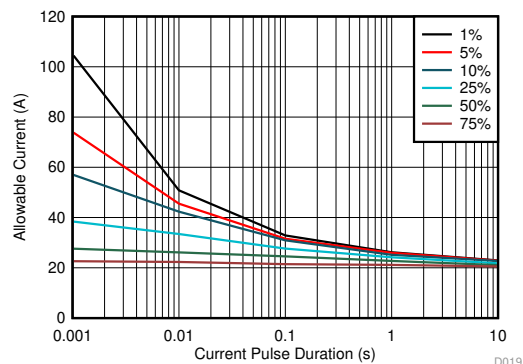
Figure 37. Maximum Repetitive Pulsed Current vs Pulse Duration
