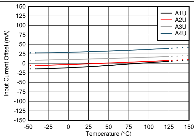
Figure 43. Offset Error Drift Across Temperature (U Variants)
