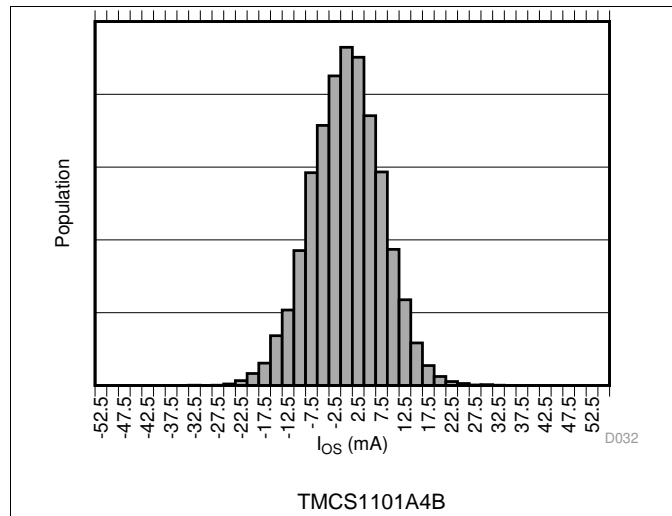
Figure 15. Input Offset Current Production Distribution
