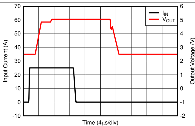
Figure 23. Voltage Output Step, Rising
