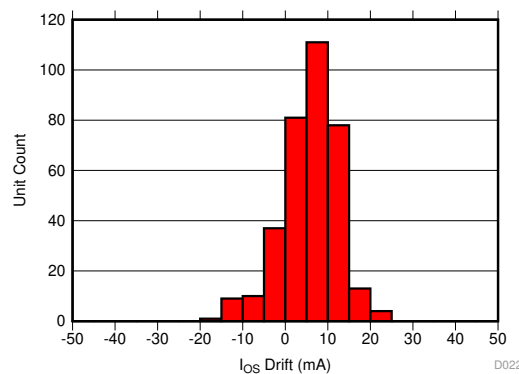
Figure 48. Input-Referred Offset Drift after AEC-Q100 High Temperature Operating Life Stress Test
