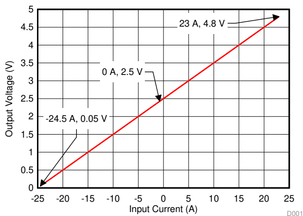
Figure 57. Application Example Design Transfer Curve
