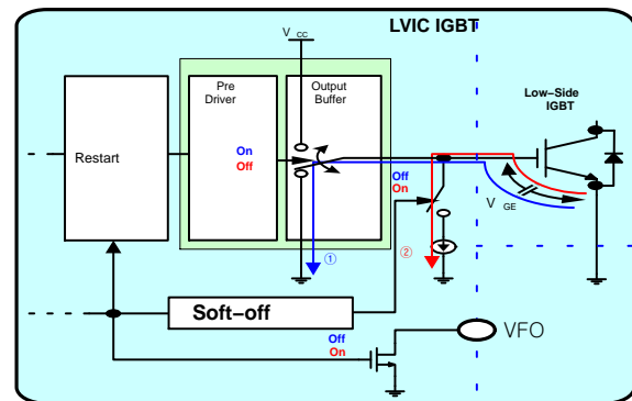
Figure 26. Operating Sequence of Soft Turn-Off
