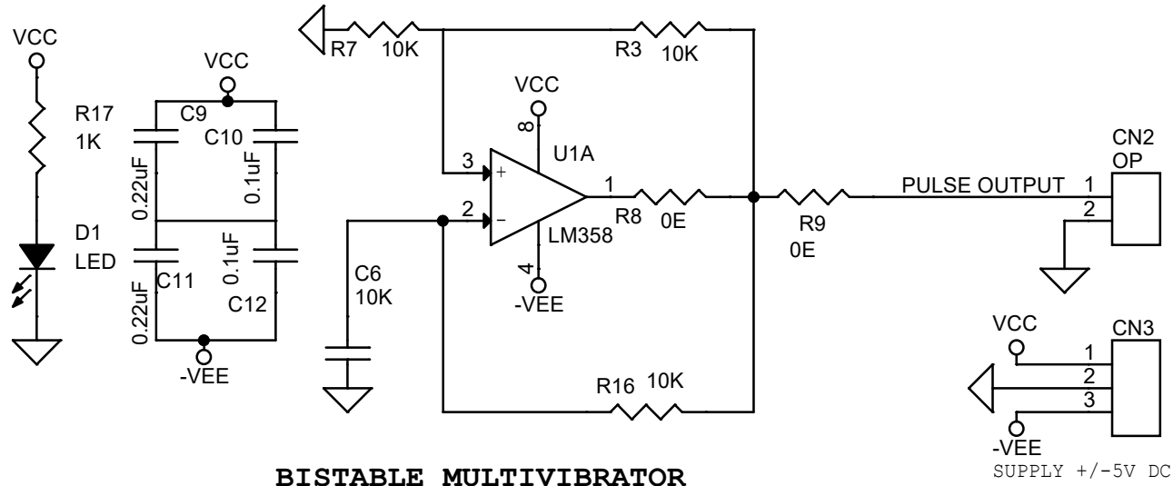
BISTABLE MULTIVIBRATOR
