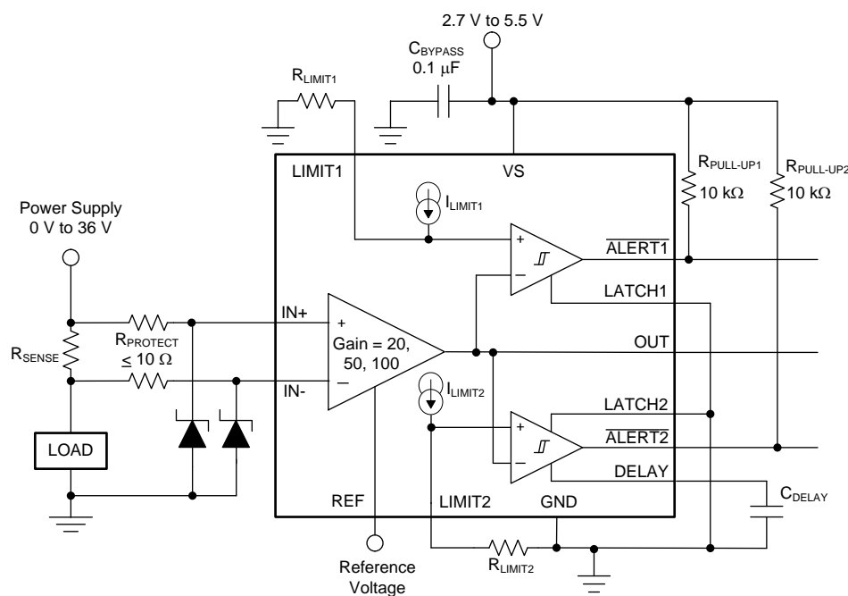
Figure 51. Transient Protection
