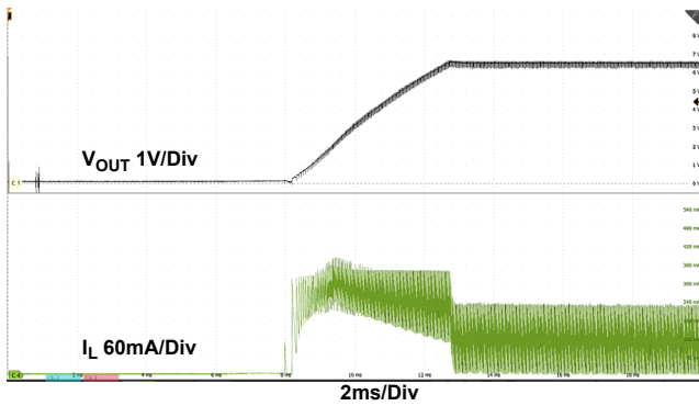
Figure 11. Startup
