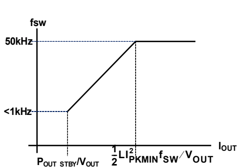
Figure 22. Switching Frequency vs I_{\text{OUT}}
